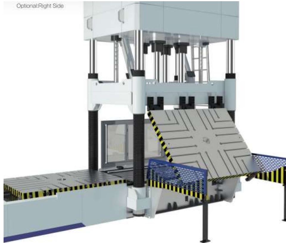
Die Spotting Machine HMG-120JM1411- 3 two way layout (right side turnover) Table Size 1400 X 1100
